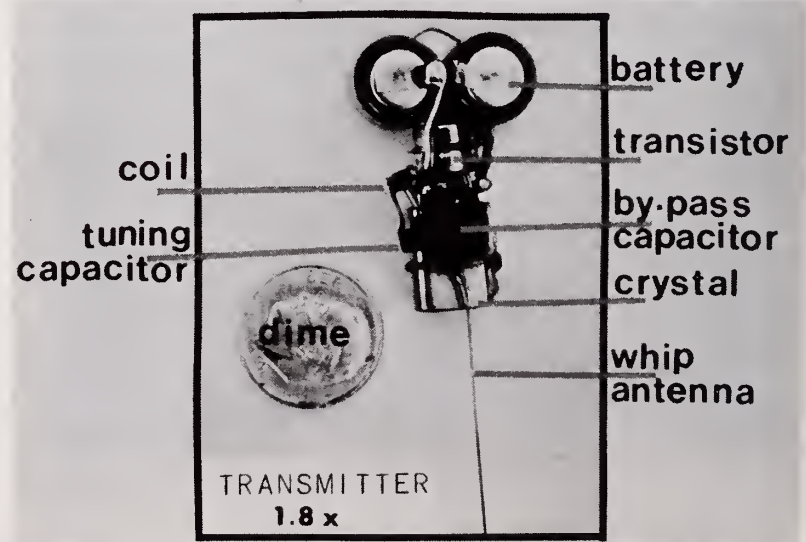
Figure 1.--Components of a 5 gram radio transmitter.
