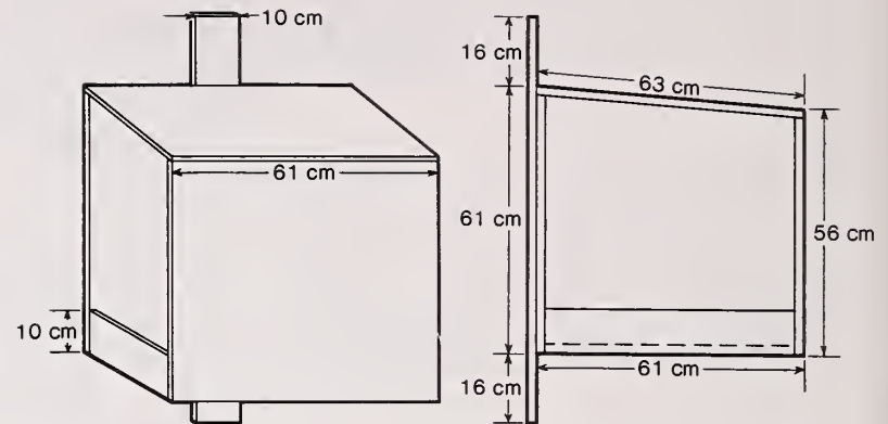
Figure 3.--Great gray owl nest box constructed of 1-cm thick plywood. The vertical support piece was a 2 x 10 cm board. Holes were drilled for 20-cm long ring-shank nails used with washers. Platforms were stained with 5 parts linseed oil and 1 part brown stain.
