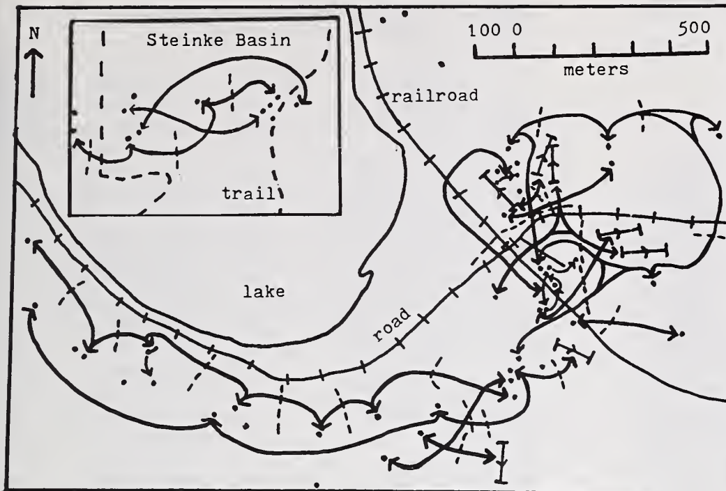
Figure 2. Map of Devil's Lake State Park, south shore area and Steinke Basin, indicating the calling records of different Saw-whet Owls and Eastern Screech-Owls on the same night with arrowpoints connected by the same line.
